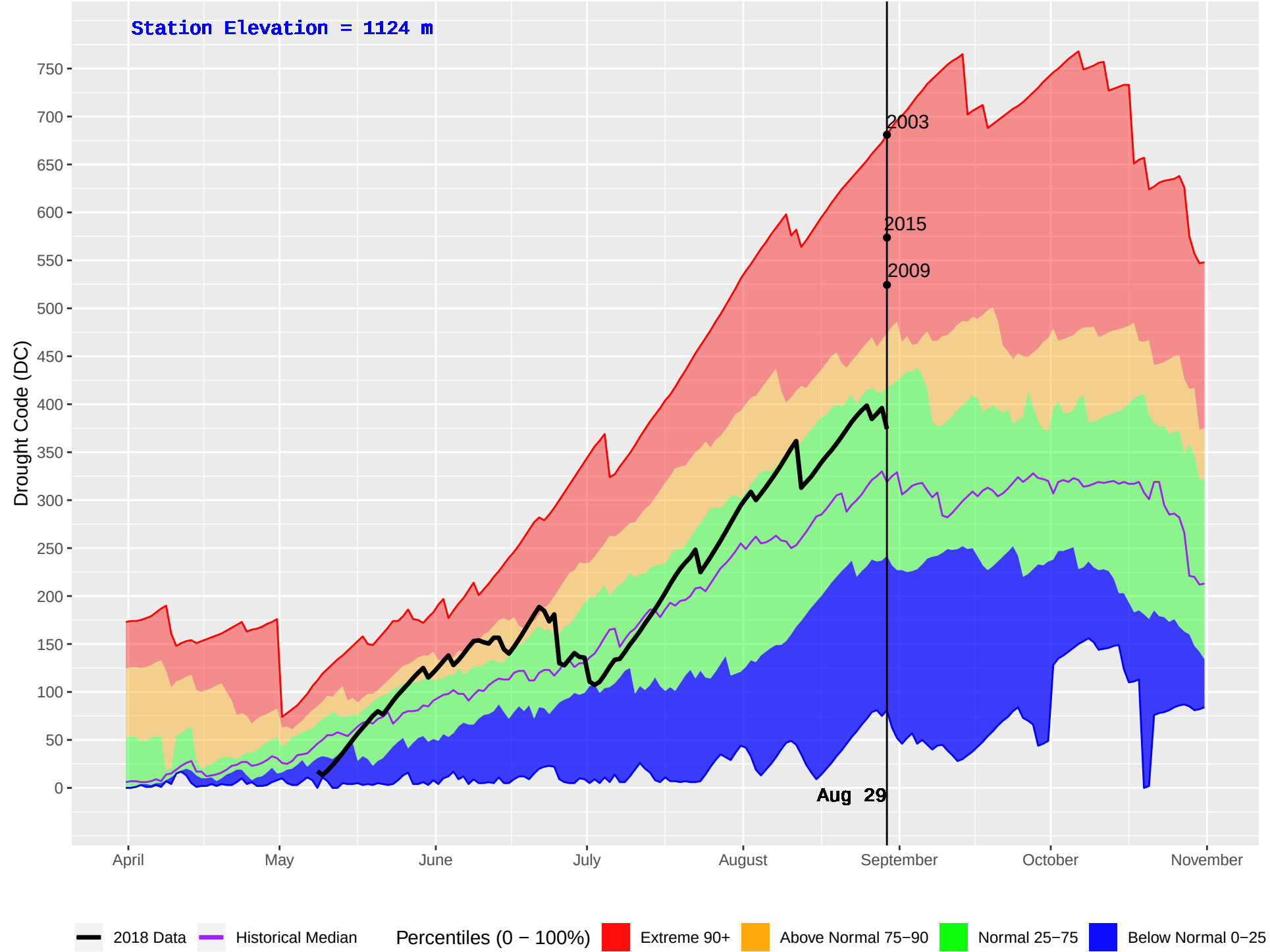
COLDSCAUR LAKE (232) : Historical (1979–2016) and Current (2018) Daily Drought Code (DC)
