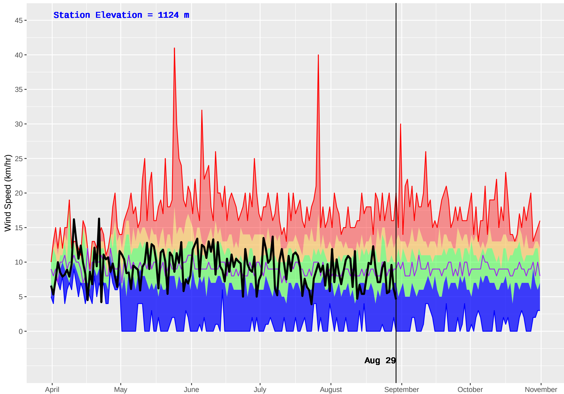
COLDSCAUR LAKE (232) : Historical (1979–2016) and Current (2018) Daily Wind Speed
