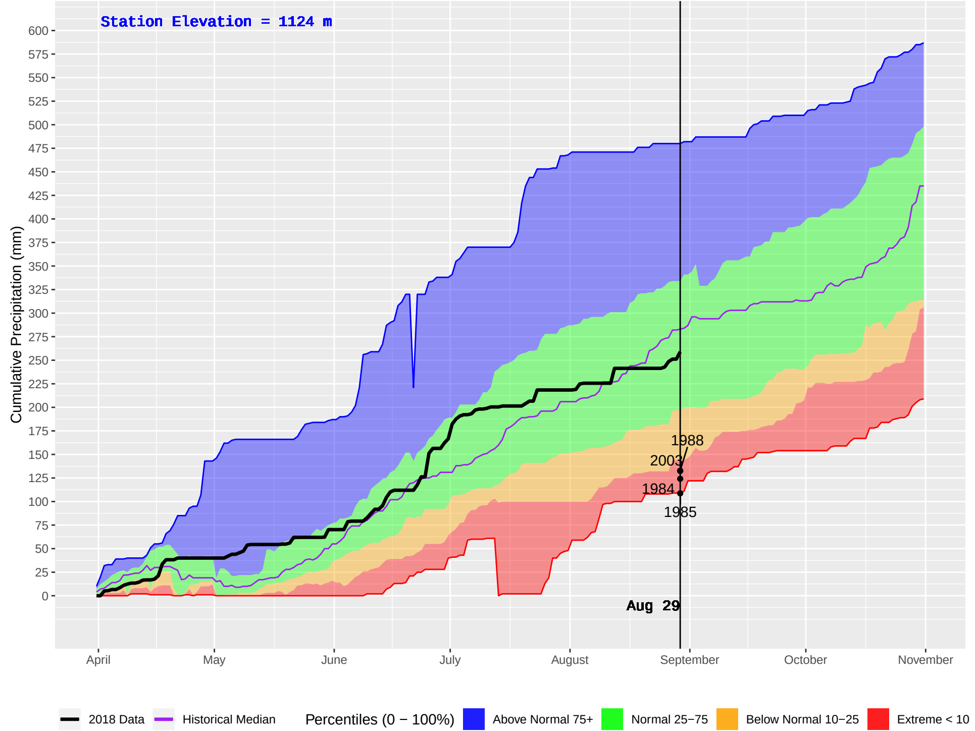
COLDSCAUR LAKE (232) : Historical (1979–2016) and Current (2018) Daily Cumulative Precipitation
