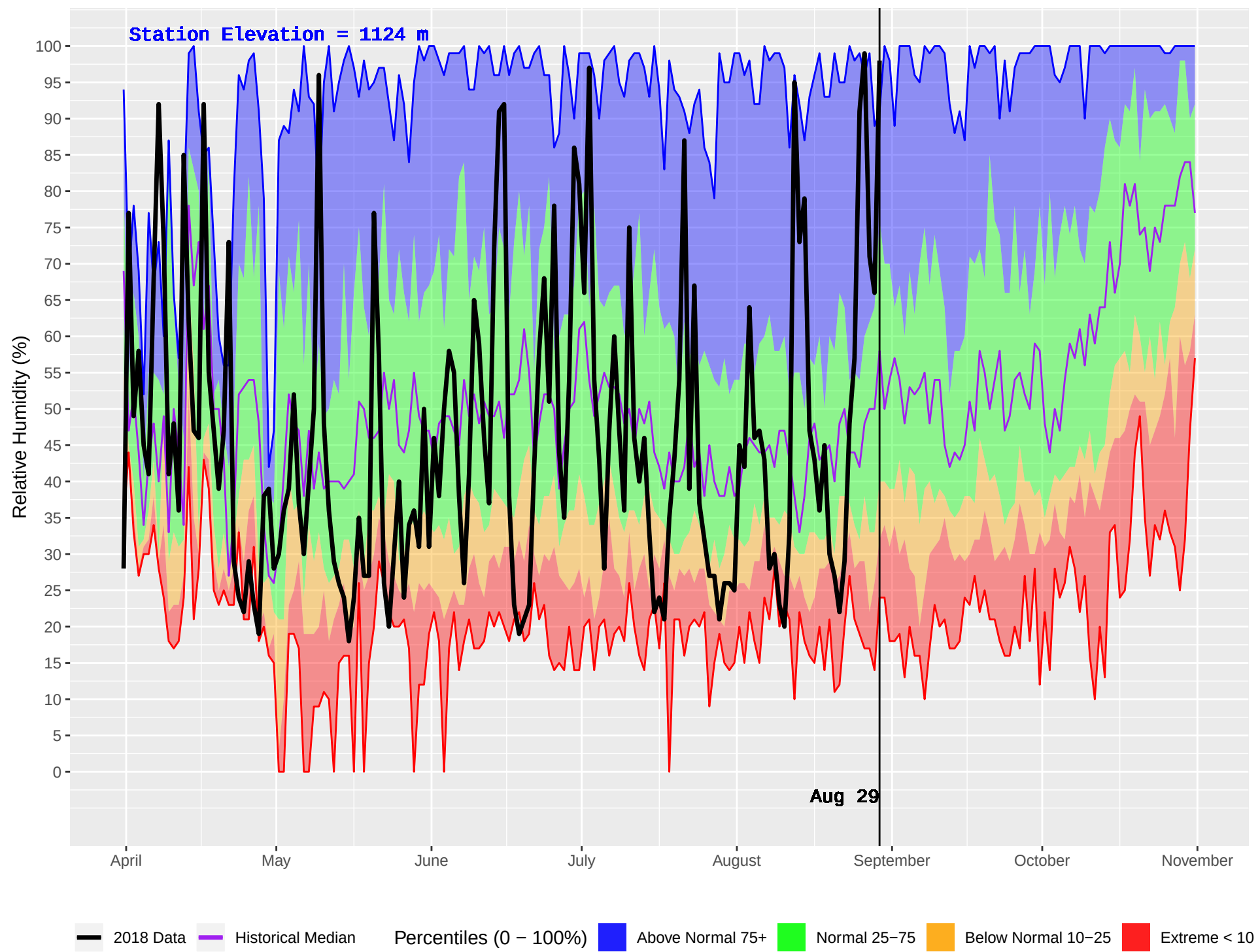
COLDSCAUR LAKE (232) : Historical (1979–2016) and Current (2018) Daily Relative Humidity
