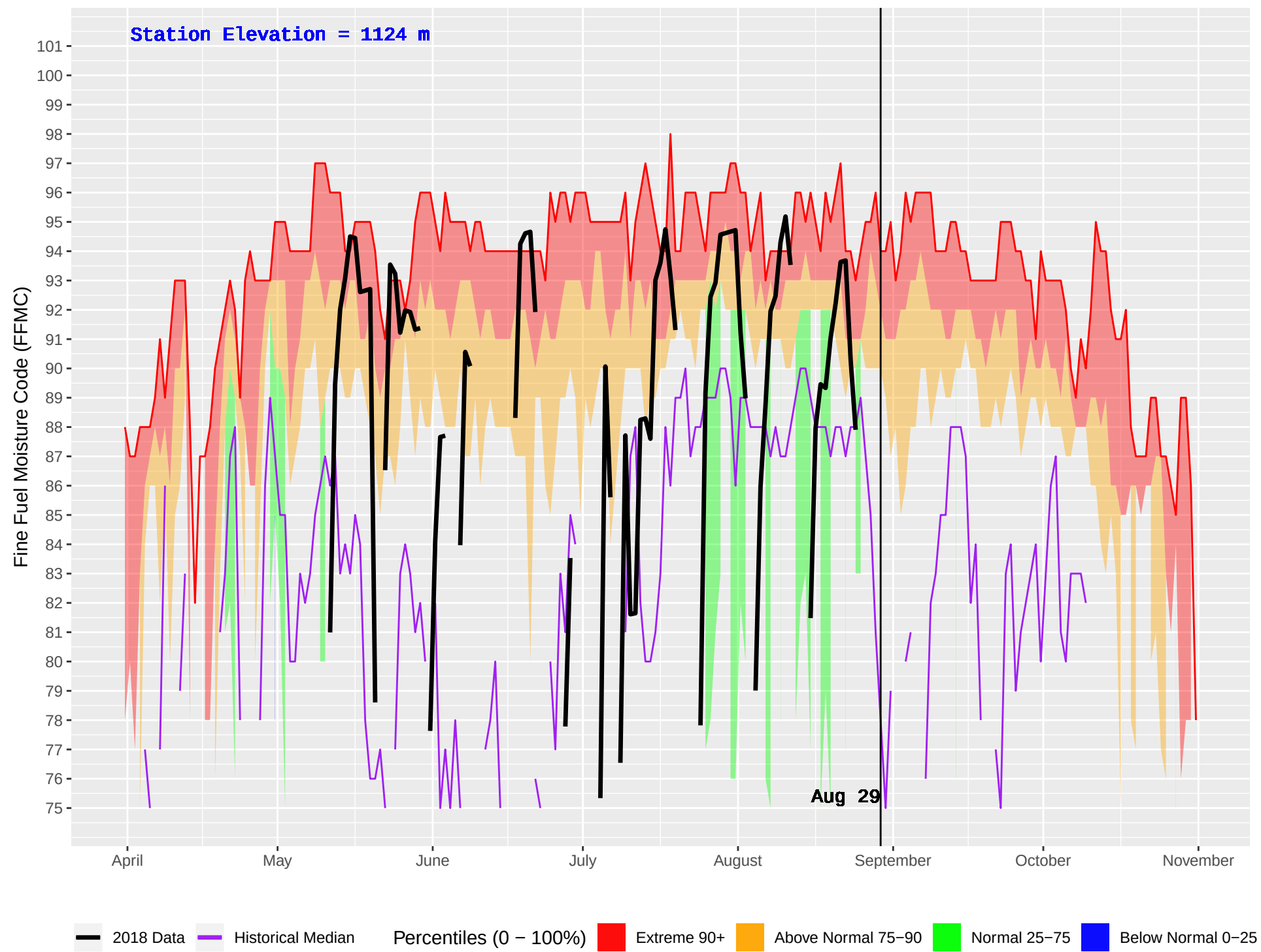
COLDSCAUR LAKE (232) : Historical (1979–2016) and Current (2018) Daily Fine Fuel Moisture Code (FFMC)
