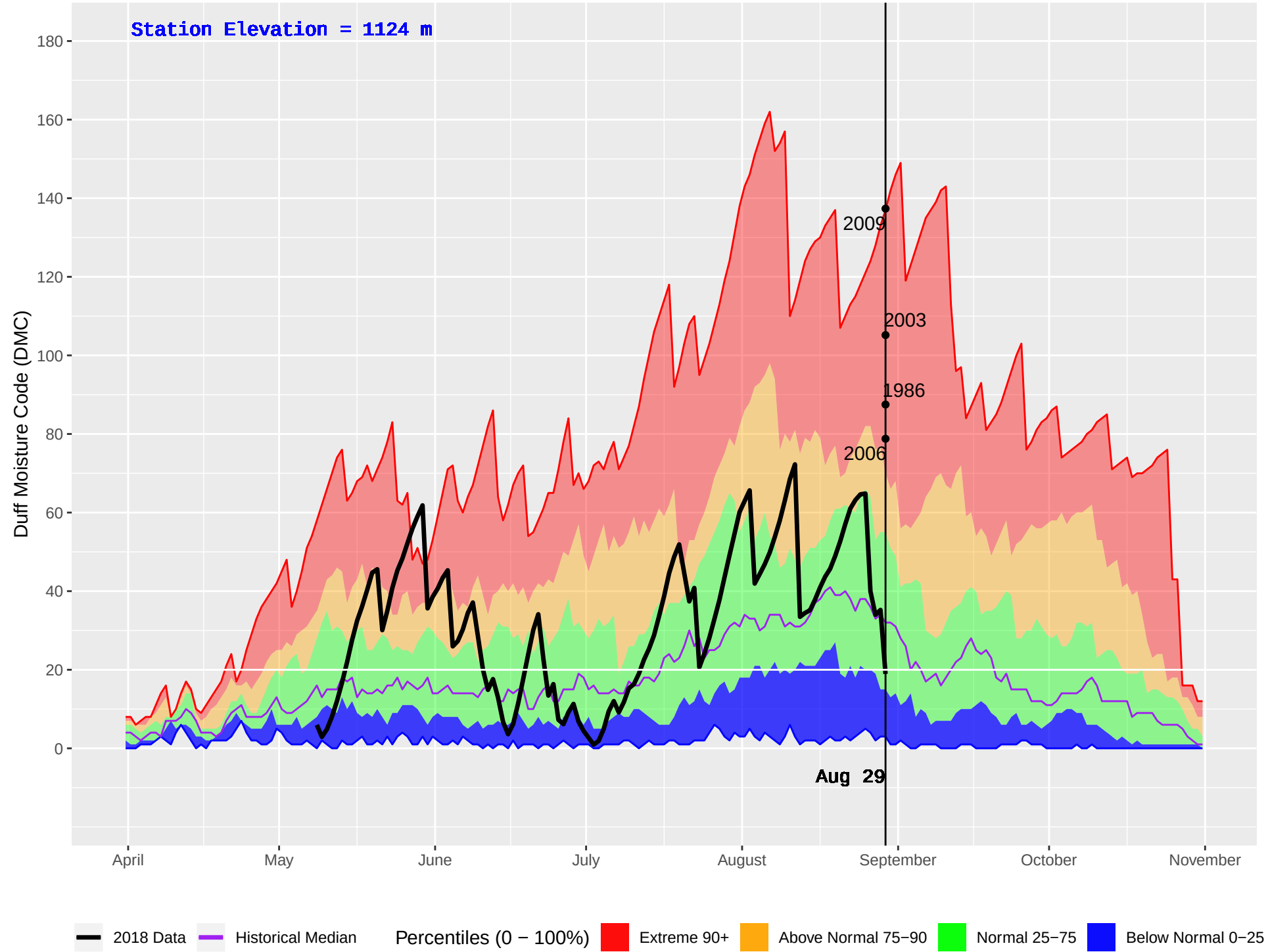
COLDSCAUR LAKE (232) : Historical (1979–2016) and Current (2018) Daily Duff Moisture Code (DMC)
