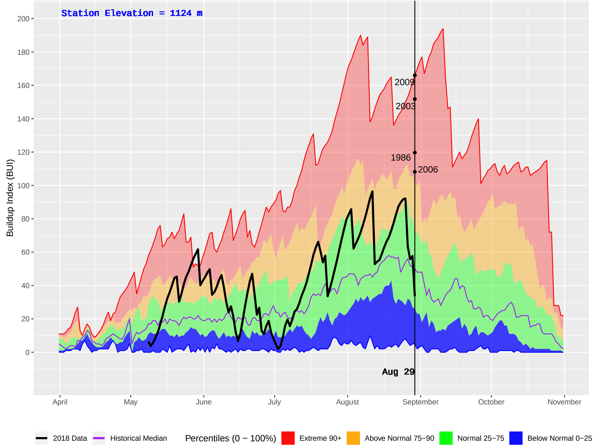
COLDSCAUR LAKE (232) : Historical (1979–2016) and Current (2018) Daily Buildup Index (BUI)
